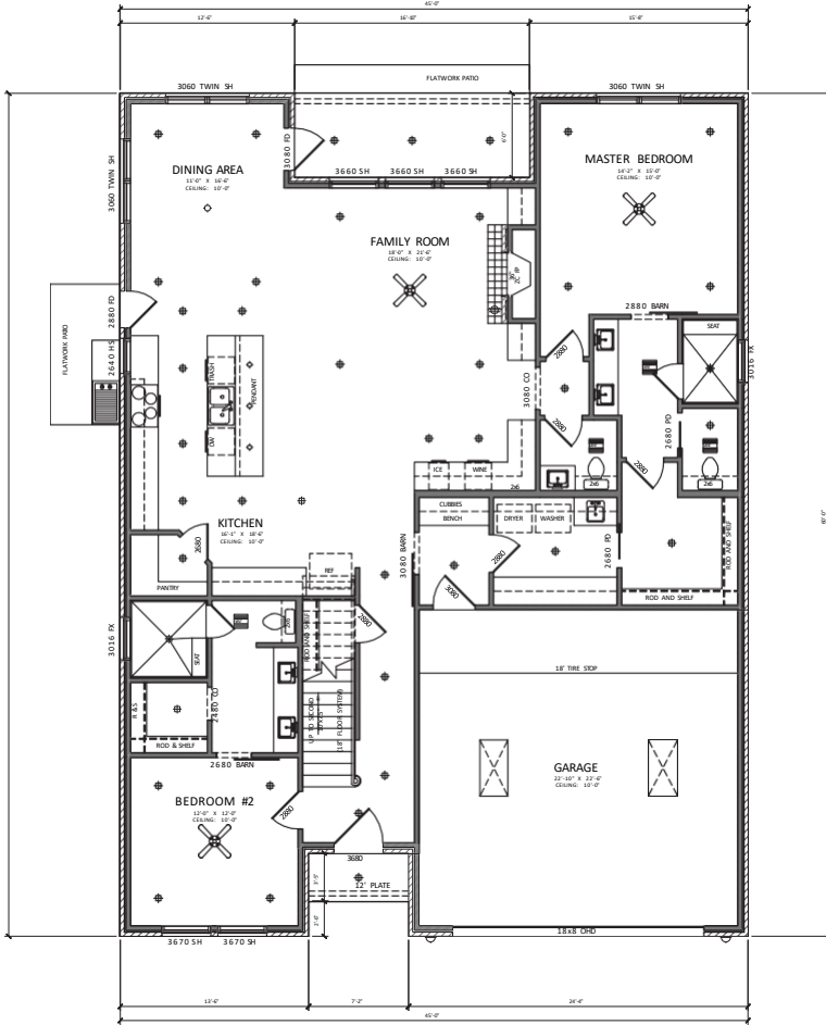
01 1ST FLOOR PLAN REFERENCE: 01A.1.1 SCALE: 1/8" = 1'-0"
