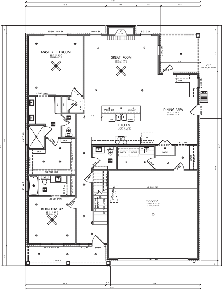
01 1ST FLOOR PLAN REFERENCE: 00A-61 SCALE: 1/8"=1'-0"
