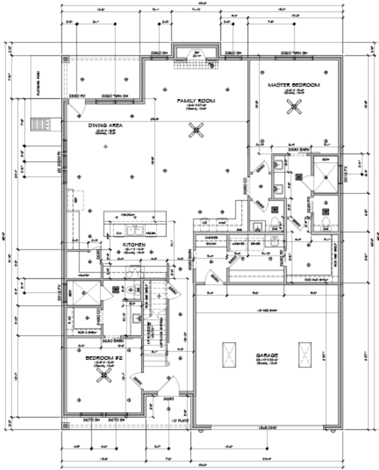
01 1ST FLOOR PLAN REFERENCE: 01-01-1 SCALE: 1/8"=1'-0"
