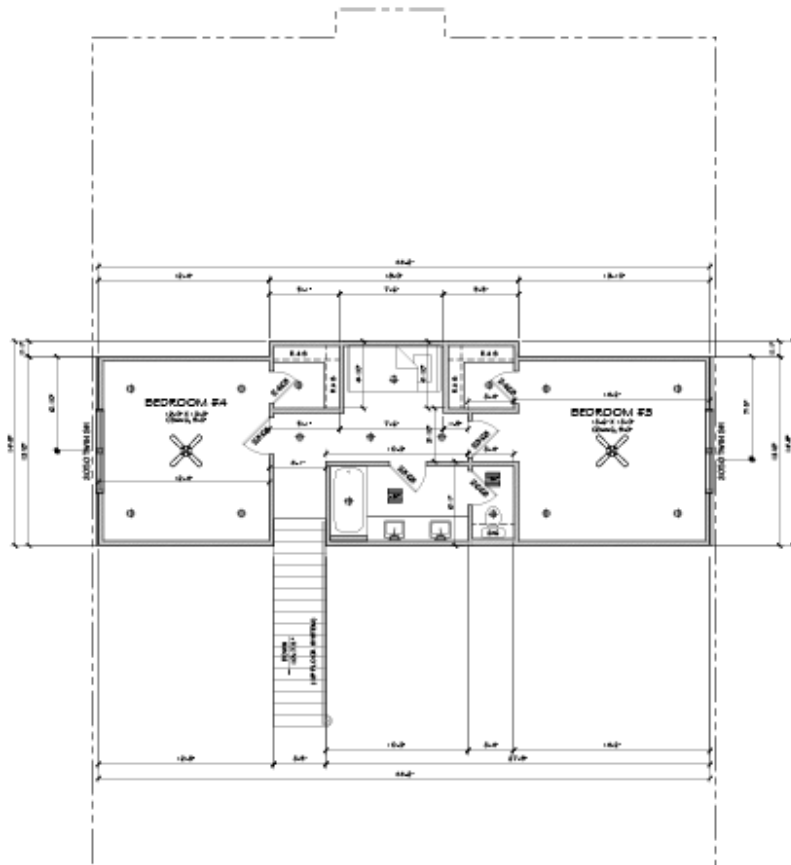
02 2ND FLOOR PLAN REFERENCE: 01-01-1 SCALE: 1/8"=1'-0"
